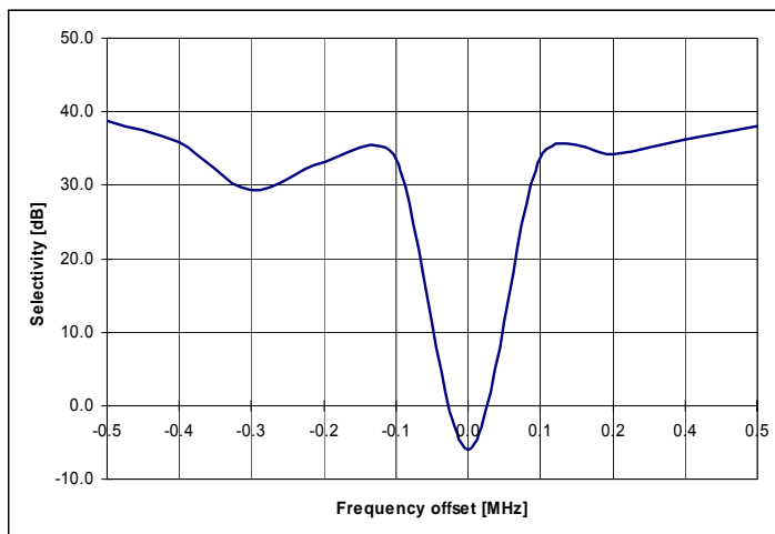
Figure 25: Typical Selectivity at 1.2 kBaud Data Rate, 868 MHz, 2-FSK, 5.2 kHz Deviation. IF Frequency is 152.3 kHz and the Digital Channel Filter Bandwidth is 58 kHz
